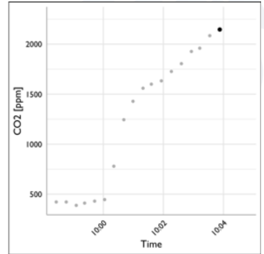
CO 2 Buildup
