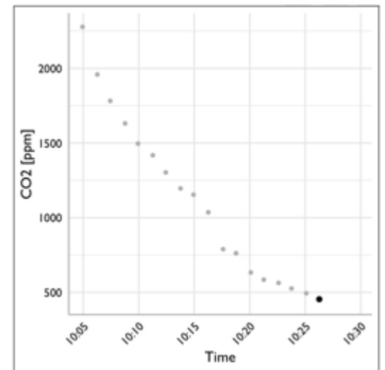
CO 2 Decay
